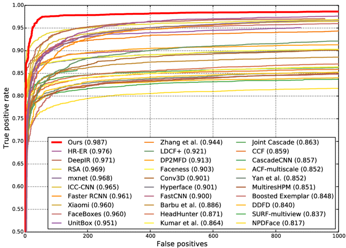
(a) Discrete ROC curves
